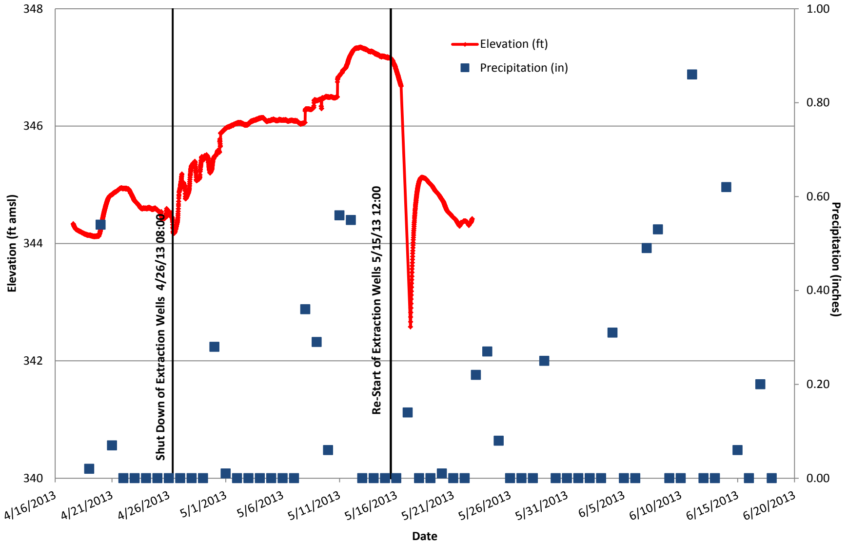
Figure 3.5-4 Building 4 Area MW-140A Vertical Extent Shutdown
